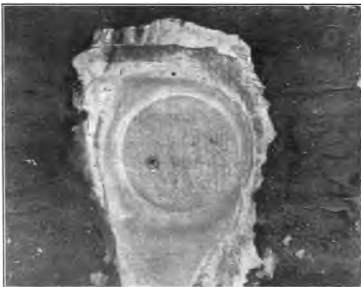
FIG. 32. — Illustrating the protection on the surface of the steel in the immediate neighborhood of a button of zinc soldered into the steel. The sphere of influence of the zinc is shown to be proscribed. (Cushman.)
