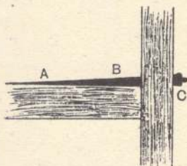
A STRAP-BOLT holding two pieces of timber together.
