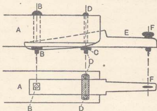
SIDE-VIEW AND UNDER-SIDE OF ARM BEDDED AND CLIPPED INTO AXLE-BED (EXBED)
