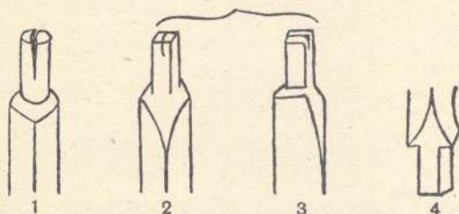
1, 2, 3, top ends or tongues of spokes, for inserting into felloes. The notch is to be spread open (thereby tightening the spoke) with a wedge driven in after the felloe has been put on. 1, round tongue; 2, square tongue, front; 3, square tongue, side. 4, foot of spoke (the tenon which holds it in the stock).
