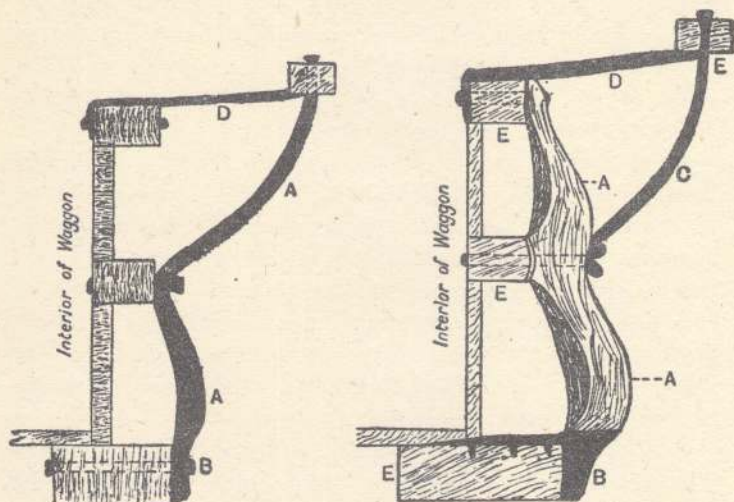
Iron Strouter (A—A) fastened with bolt (B) to main "side" of waggon or cart. It forms a stay for the outrave and supports the copse (D).
