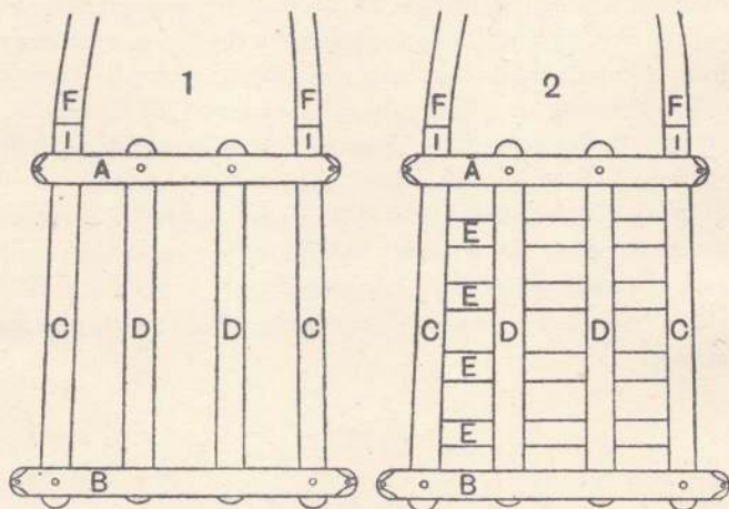
BOTTOM FRAME-WORK OF TWO-WHEELED CARTS
