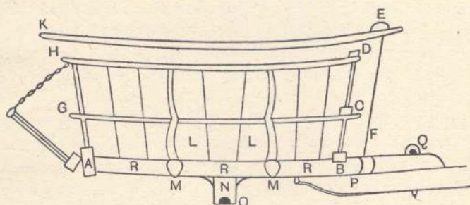
SIDE ELEVATION OF RAVED CART, WITH TAILBOARD LET DOWN
