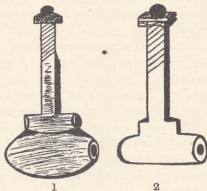
1, barrel eye; 2, ordinary eye.
