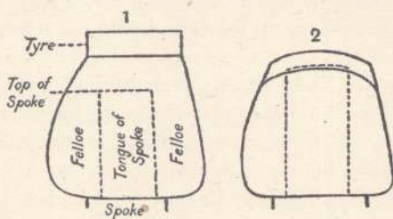
1, Section of new wheel-rim with new tyre; 2, section of worn wheel-rim with old tyre, chafing upon tongue of spoke.
